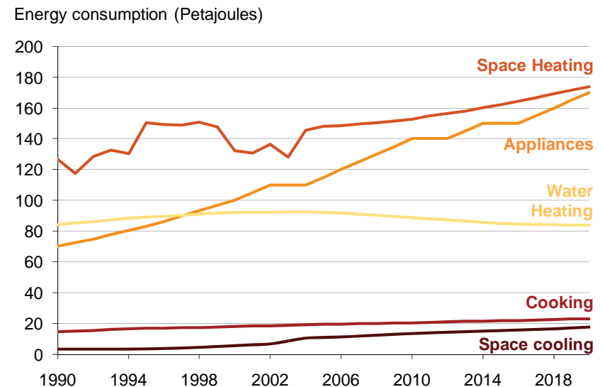
Figure 7.3 Trends in total Australian household energy consumption by major end use
