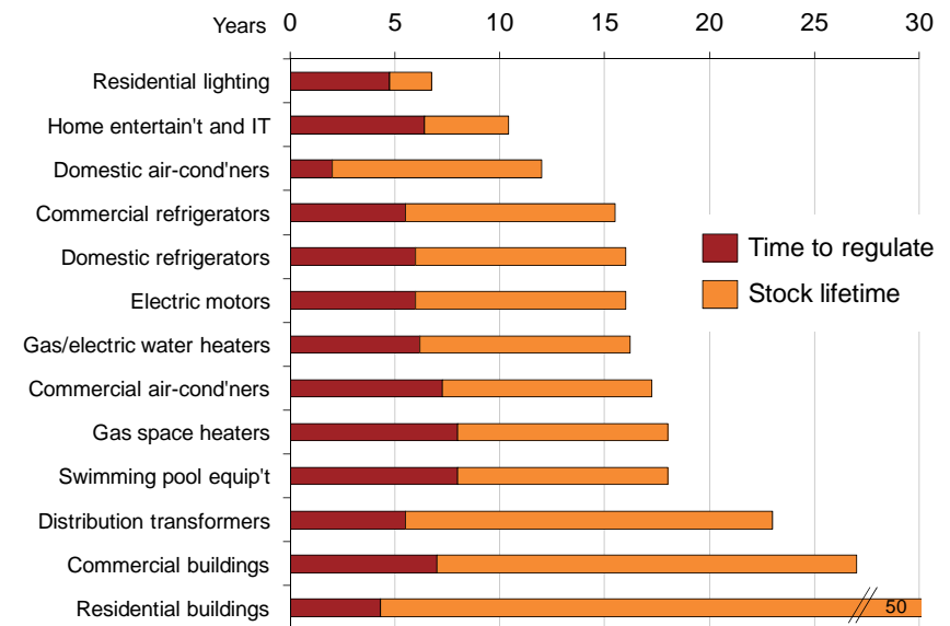
Figure 7.2 Time to implement Australian energy efficiency standards
